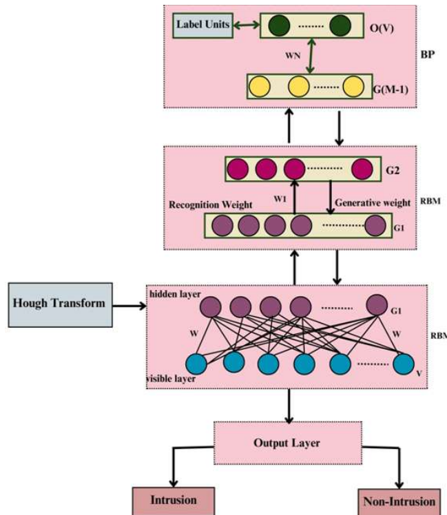
Figure 3: HT-DBN model
